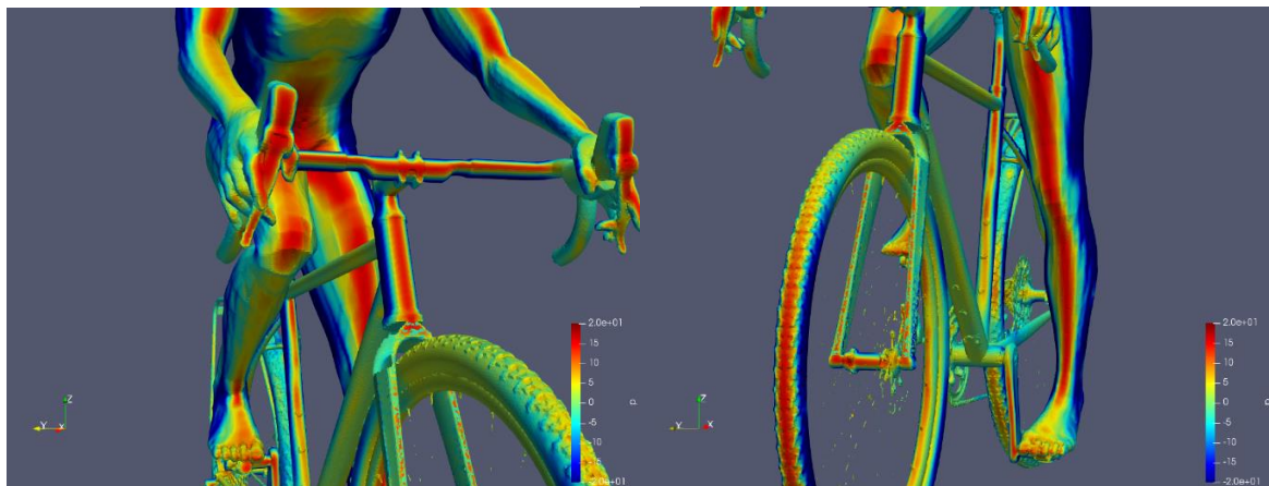
Figure 1. CFD analysis, images show surface pressure of the left and right lower extremity during cycling
