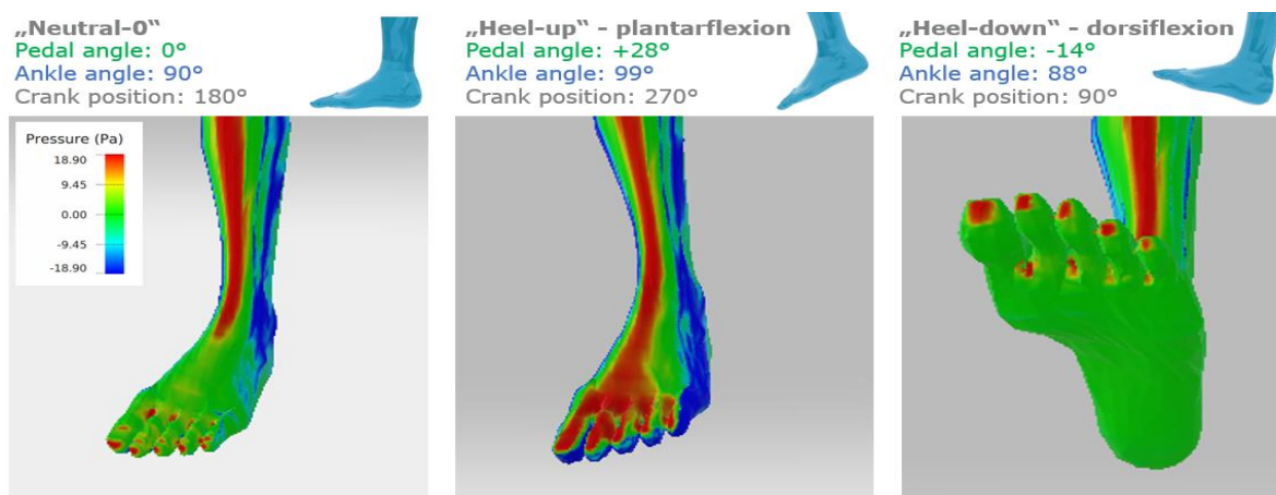
Figure 2. Surface pressure depending on pedal (orientation) angle; red colour indicates high surface pressure especially around the toe and the dorsum region of the foot
