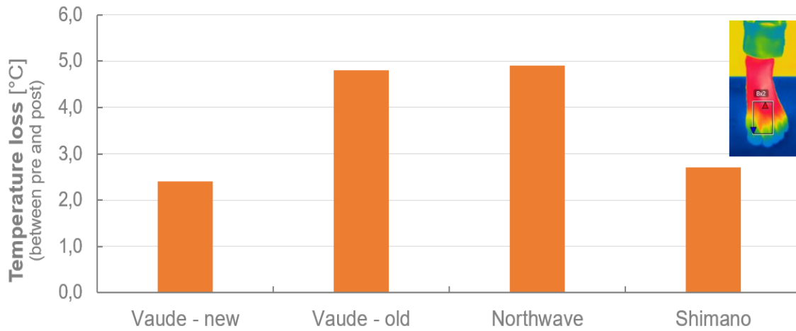
Figure 5. Temperature loss (difference) between pre and post measurements without shoes; Measurement area: dorsal region of the foot as shown in the thermal image (rectangle)
