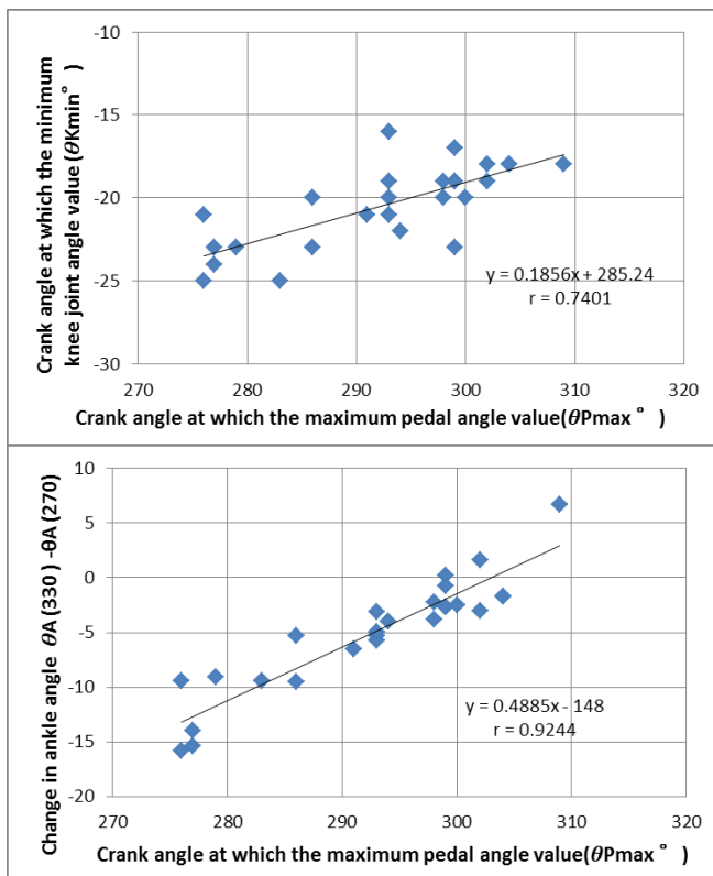
Figure 2. Relationship between hip/knee joint interaction and ankle joint movement from the crank angle corresponding with maximum pedal angle.
