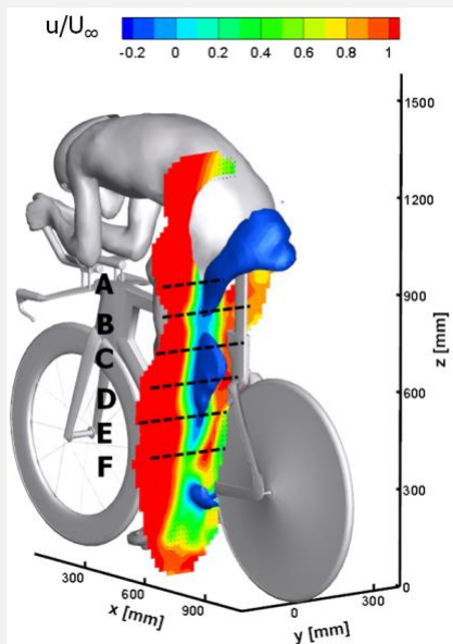
Figure 1. Cross-section of mean non-dimensional streamwise velocity in the near-wake of the stretched leg obtained at U_\infty = 5 m/s. The dark blue iso-surface depicts a zero level of streamwise velocity.
