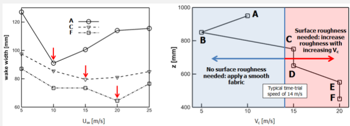
Figure 2. Wake width (left; the red arrows indicate the critical velocities at the different sections) and critical velocity (right) along the leg
